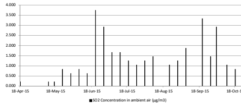
SO 2 Concentration at Doramadala in µg/m 3 from App to Oct 2015
