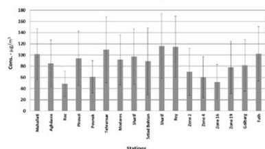
PM10 annual average of Tehran air quality monitoring stations, March 2013-Feb 2014
