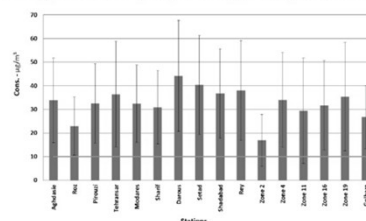
PM2.5 annual average of Tehran air quality monitoring stations, March 2013-Feb 2014
