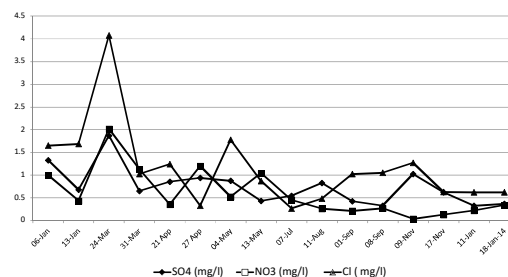
Concentration of Anions from Jan 2013 to Jan 2014
