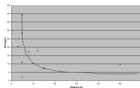
Relationship Between \text{NO}_2 Concentration and Distance from Main Road
