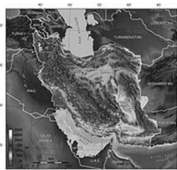
Topographic Map
